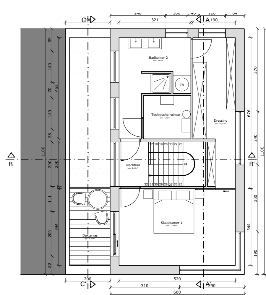
Grondplan +2 opp. 45,10m 2
