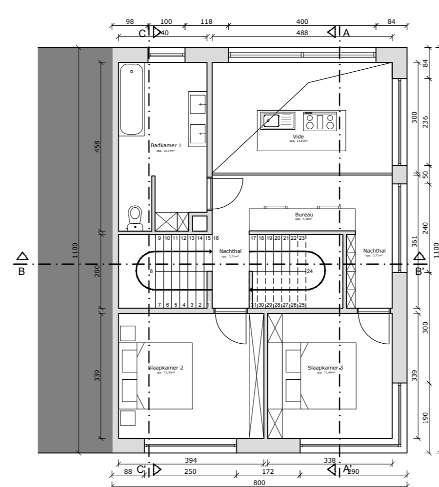
Grondplan +1 opp. 51,61m 2
